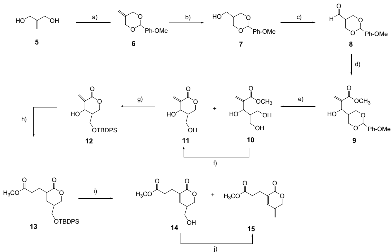
Scheme 4. Reagents and conditions: (a) anisaldehyde, TsOH; 93%; (b) (1) 9-borabicyclo[3.3.1]nonane (9-BBN), (2) NaOH, H 2 O 2 ; 78%; (c) (COCl) 2 , DMSO, triethylamine; 86%; (d) methyl acrylate, 1,4-diazabicyclo[2.2.2]octane (DABCO), triethanolamine, La(OTf) 3 , [bmim][PF 6 ]; 60%; (e) 0.01 N H 2 SO 4 ; (10:11 = 1:2); (f) Bu 4 NF (TBAF); 72% (from 9 to 11); (g) ( t -Bu)Ph 2 SiCl (TBDPS-Cl), DMAP, triethylamine; 65%; (h) MeC(OMe) 3 , propionic acid; 76%; (i) Bu 4 NF (TBAF); 54% (from 13 to 14); 34% (from 13 to 15); (j) (1) TsCl, (2) 1,8-diazabicyclo[5.4.0]undec-7-ene (DBU); 84%.
