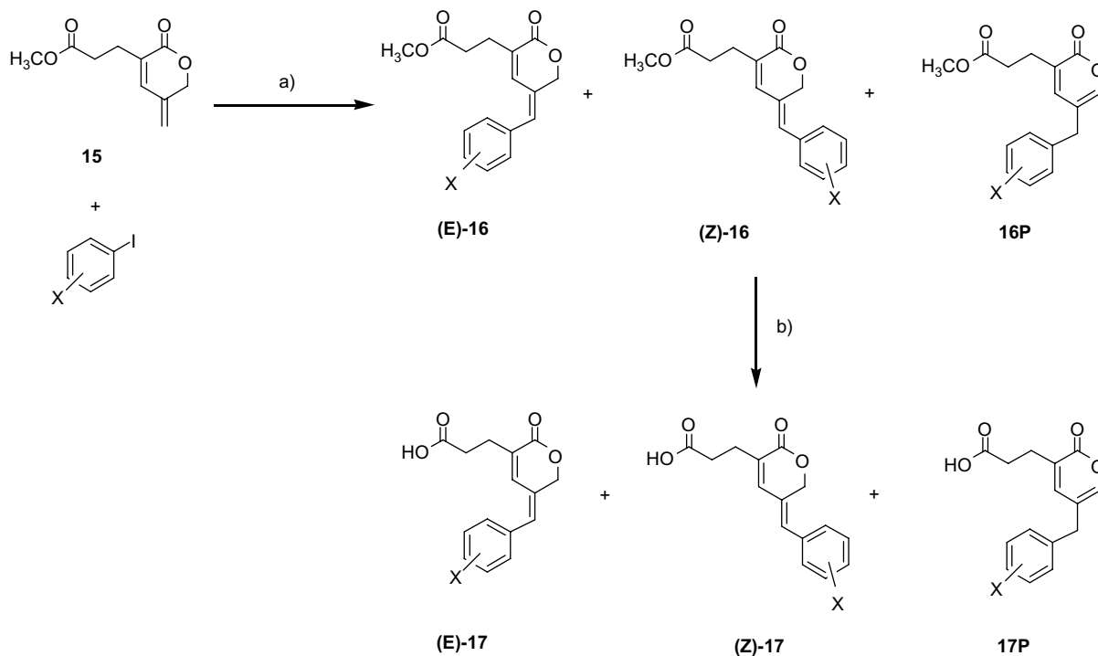
Scheme 5. Reagents and conditions: (a) Pd(OAc) 2 , PPh 3 , AgOAc; (b) LiOH/H 2 O, MeOH/H 2 O.
